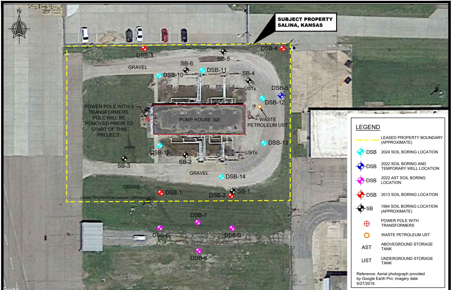
FIGURE 2 PROPERTY BOUNDARY MAP AND SOIL BORING LOCATION MAP
