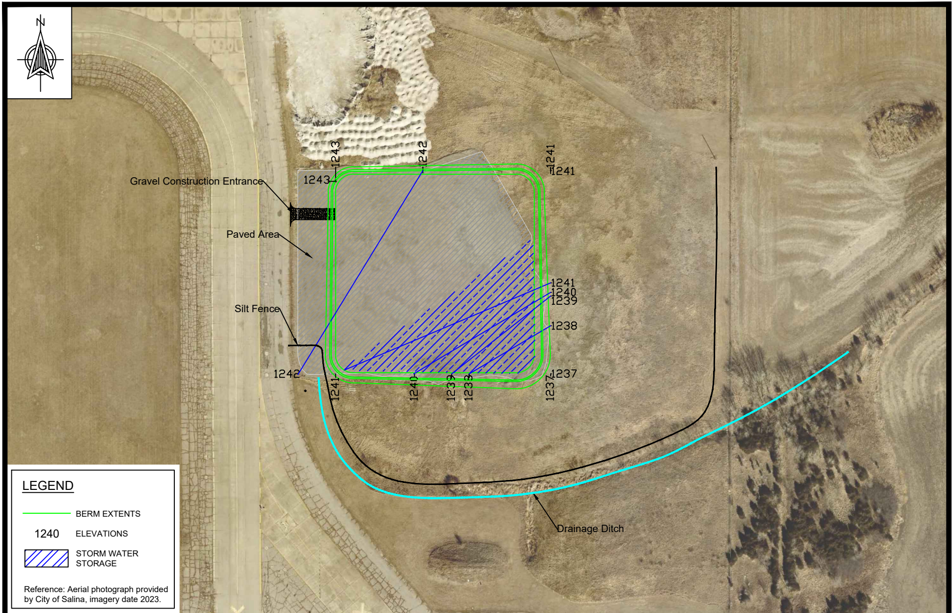
FIGURE 7 LAND FARM PLAN VIEW DETAIL
