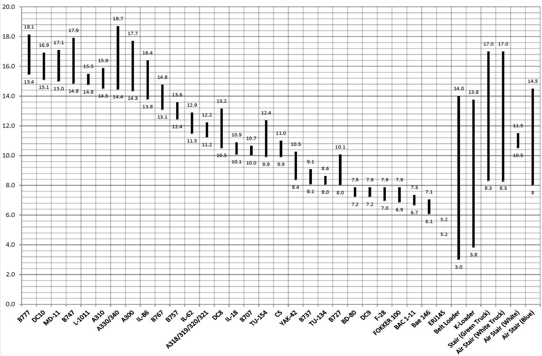
Aircraft Door Sill Heights in Feet (Minimum to Maximum)
